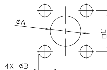
Mounting Dimension
